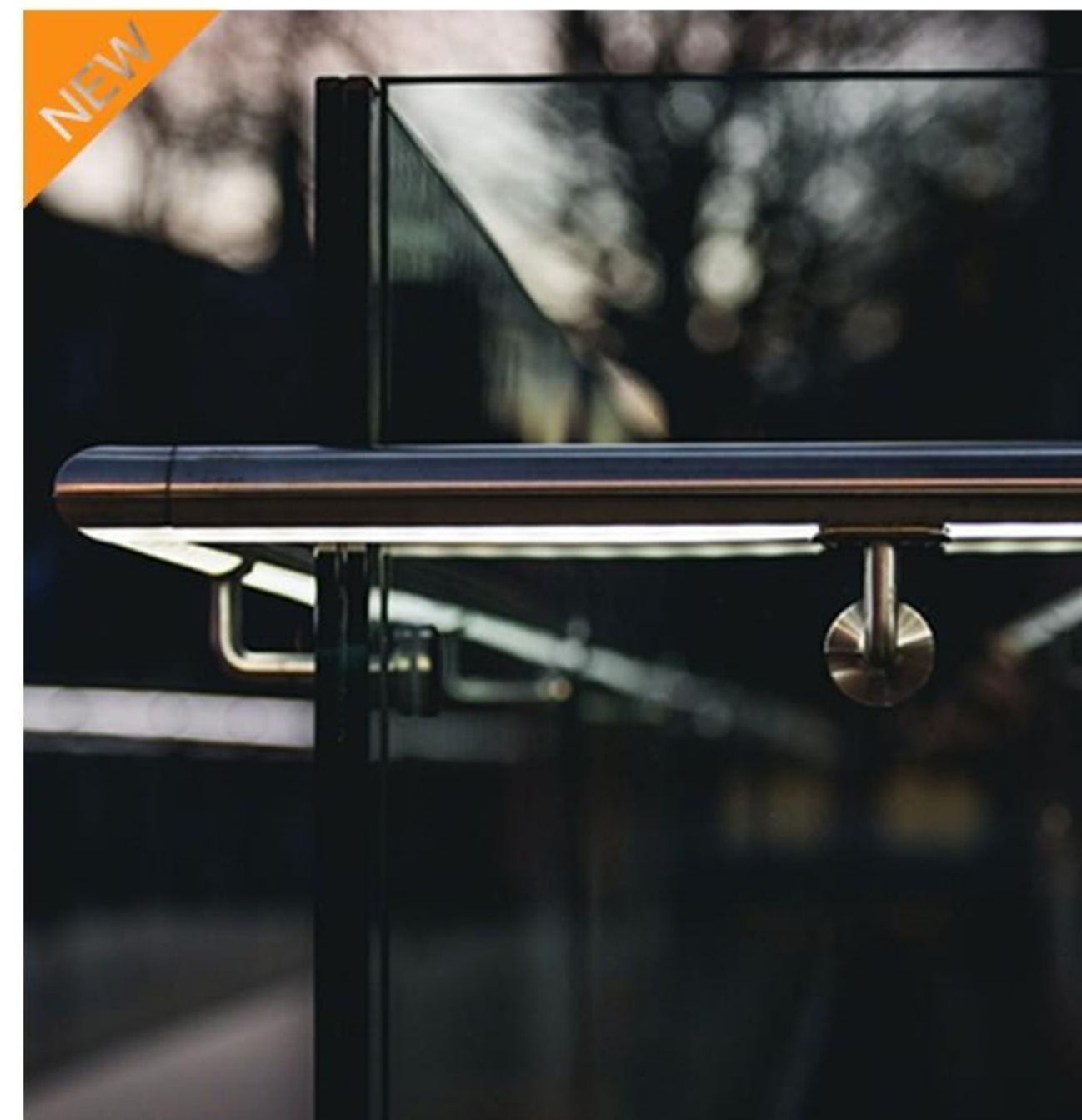
the wall holder of a hand-rail of Ø50.8mm "house-keeper"
